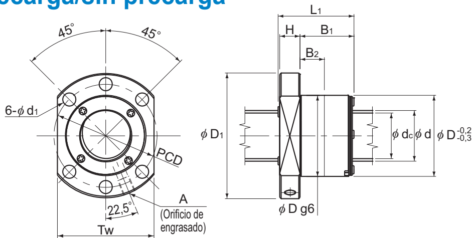
SDA3110V/3112V/3116V/3120V/3132V
