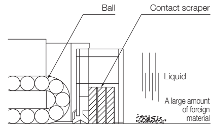
Structural Drawing
