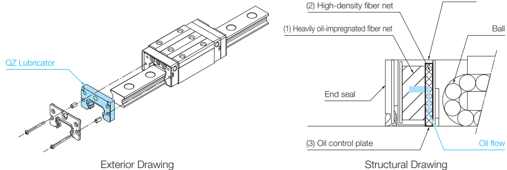
Overall LM Block Length Dimension with QZ Lubricator and Seals Attached
