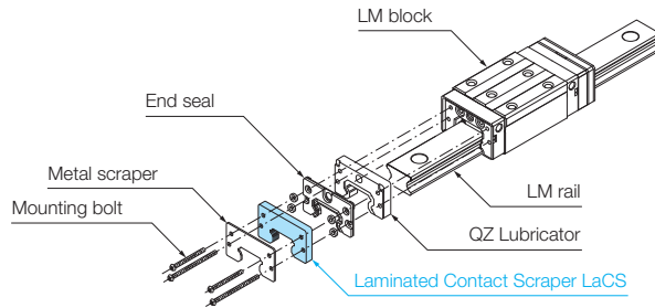
Exterior Drawing
