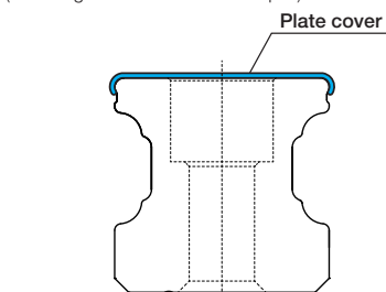
Plate Cover Installation and Cross-Section (The image is an illustrative example.)
