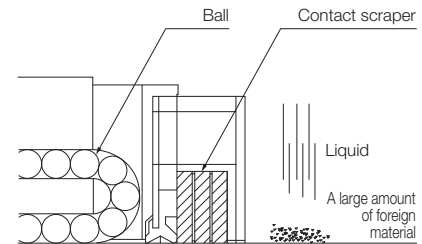
Structural Drawing
