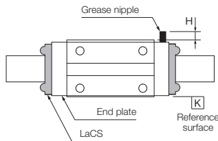
Location for mounting the side grease nipple
